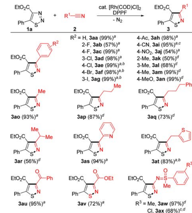
Scheme 2. Nitrile Substrate Scope a
