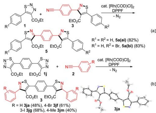
Scheme 5. Synthesis of Pentaoligomeric Arylene Compounds
