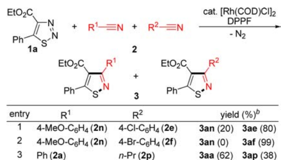
Scheme 4. Competition Experiments between Various Benzonitriles a
