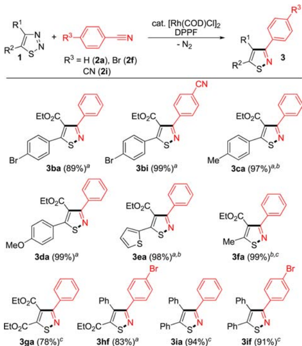
Scheme 3. Thiadiazole Substrate Scope a
