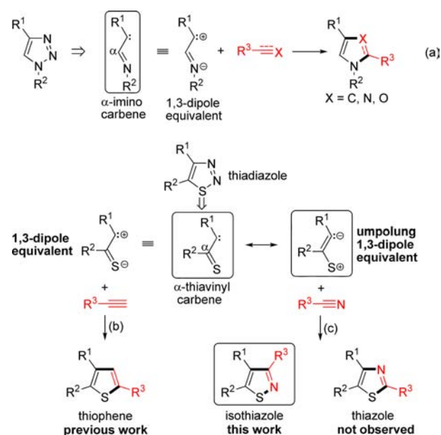
Scheme 1. 1,3-Dipole Equivalents Generated from Triazoles and Thiadiazoles
