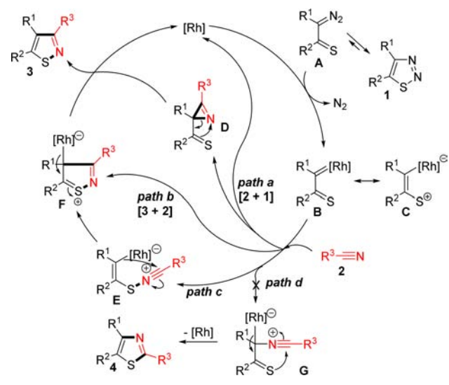
Scheme 6. Possible Mechanism
